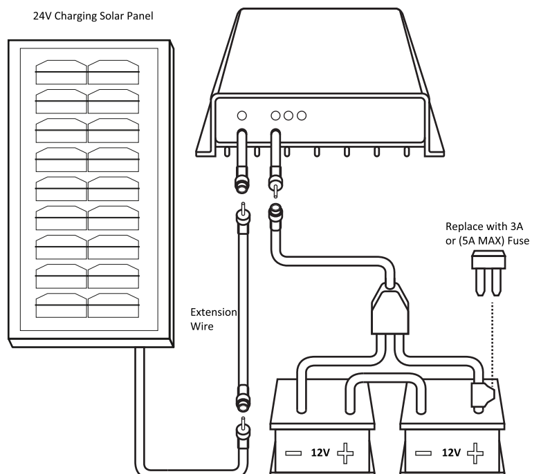
24V Connection Diagram
