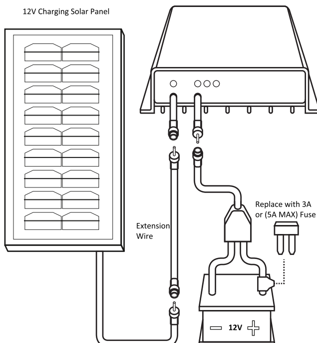
12V Connection Diagram
